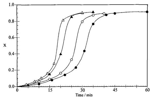
Figure 5 Variation of the conversion x versus time histories with the initiator concentration. Initial monomer concentration = 0.4M. Polymerization temperature = 75°C. [K_2S_2O_8] \times 10^3 = 0.25 (●), 0.50 (○), 1.00 (▲), and 1.50M (△).
