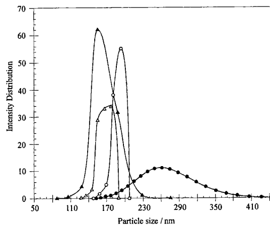
Figure 3 Dependence of the particle size distribution of the lattices on the polymerization temperature. See Figure 2 caption for the reaction conditions. Polymerization temperature = 60^\circ C (●), 65^\circ C (○), 70^\circ C (▲), and 75^\circ C (△).
